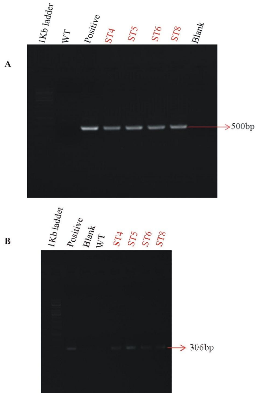
Fig. 7: Agarose gel electrophoresis of PCR amplified genomic DNA of T 1 generation finger millet single gene transgenic ( OsSOS1 ) plants
